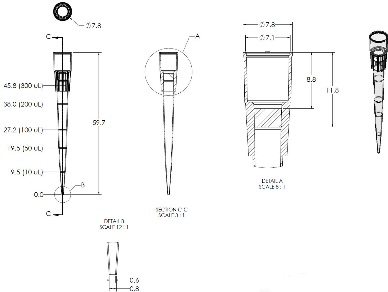
WB 6050 TripleA 300 \mu L LTS Compatible Tips Racked, Sterile – Filtered
